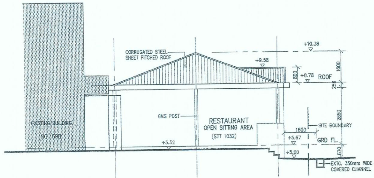
WEST ELEVATION
