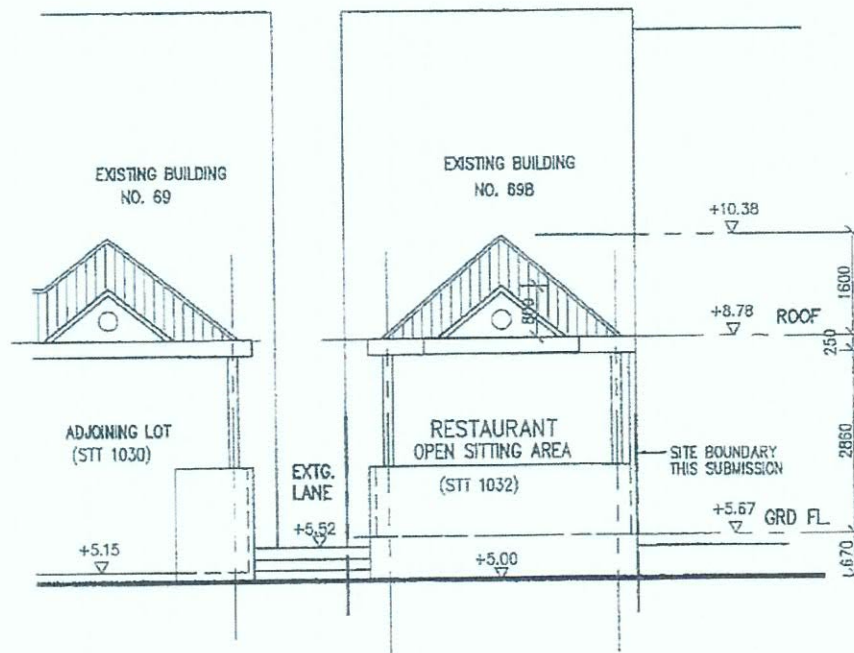
SOUTH ELEVATION
