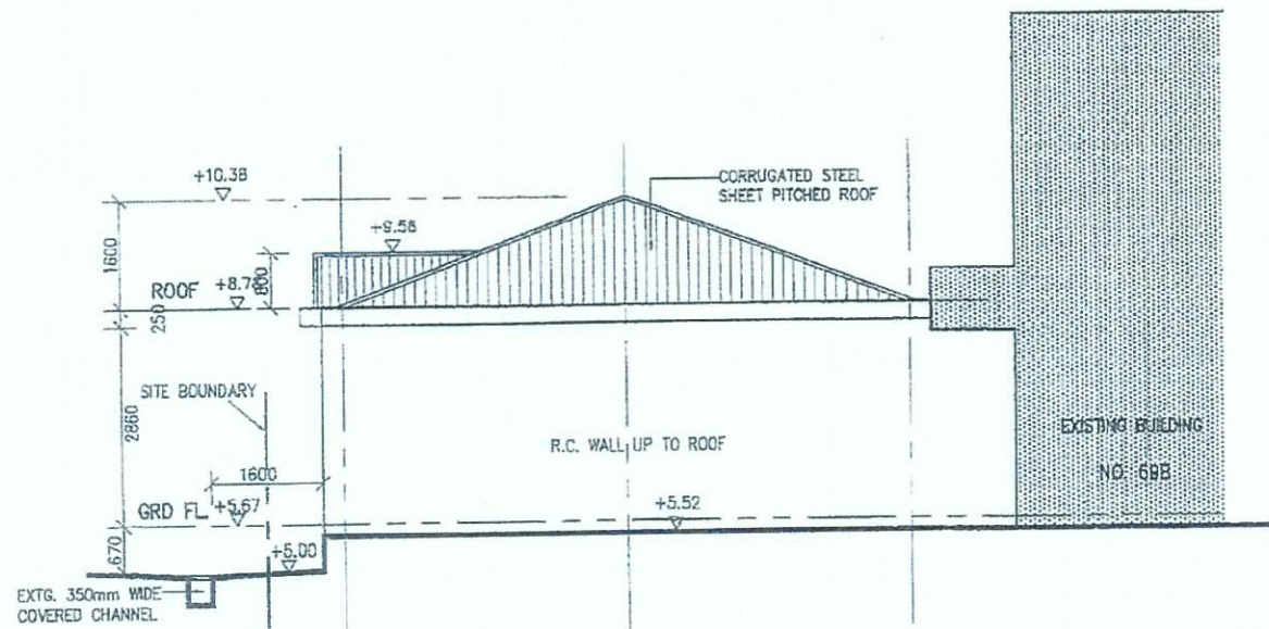
EAST ELEVATION
